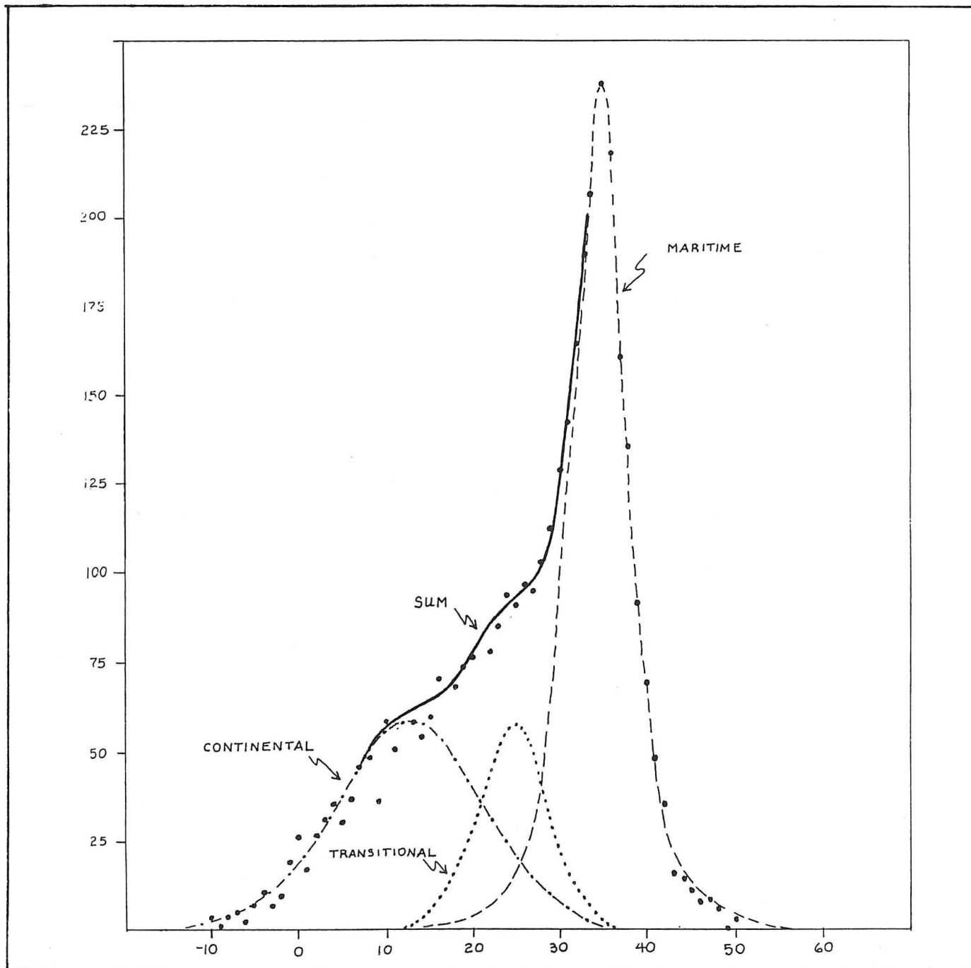
Figure 3. The approximate normal curves for the daily mean temperatures ( ^{\circ}\text{F} ) of the three climatic regimes and their sum. The observed distribution is displayed with dots.
