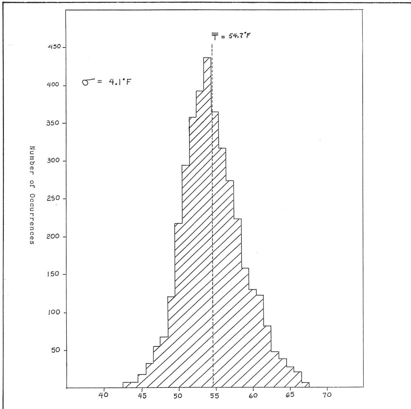
Figure 1. Distribution of Summer (June, July, August) Daily Mean Temperatures ( ^{\circ}\text{F} ) for the Years 1943 - 1984.
