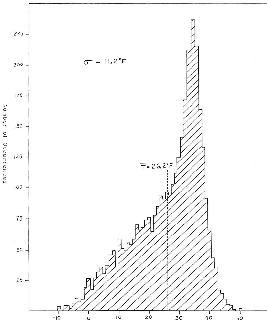
Figure 2. Distribution of Winter (December, January, February) Daily Mean Temperatures ( ^{\circ}\text{F} ) for the Years 1943 - 1984.
