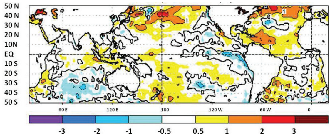
Fig. 4. A sample sea surface temperature anomaly ( ^{\circ}\text{C} ) map from the month of September 2005 (source: Climate Prediction Center: Climate Diagnostics Bulletin). The anomalies are relative to the 1971 – 2000 base period.
