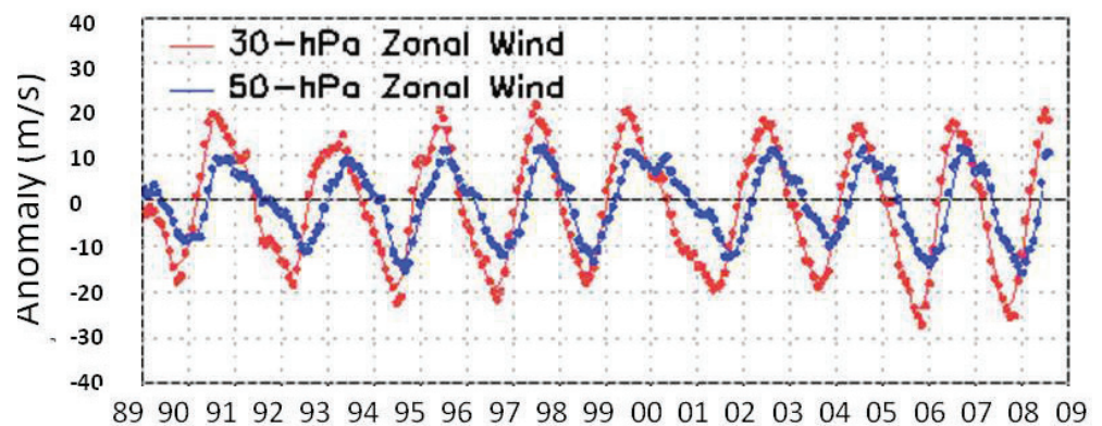
Fig. 5. A time series of 30 hPa (red) and 50 hPa (blue) winds for the tropics ( 5^{\circ}\text{N} to 5^{\circ}\text{S} ) covering approximately a 20 year period (source: Climate Prediction Center).
