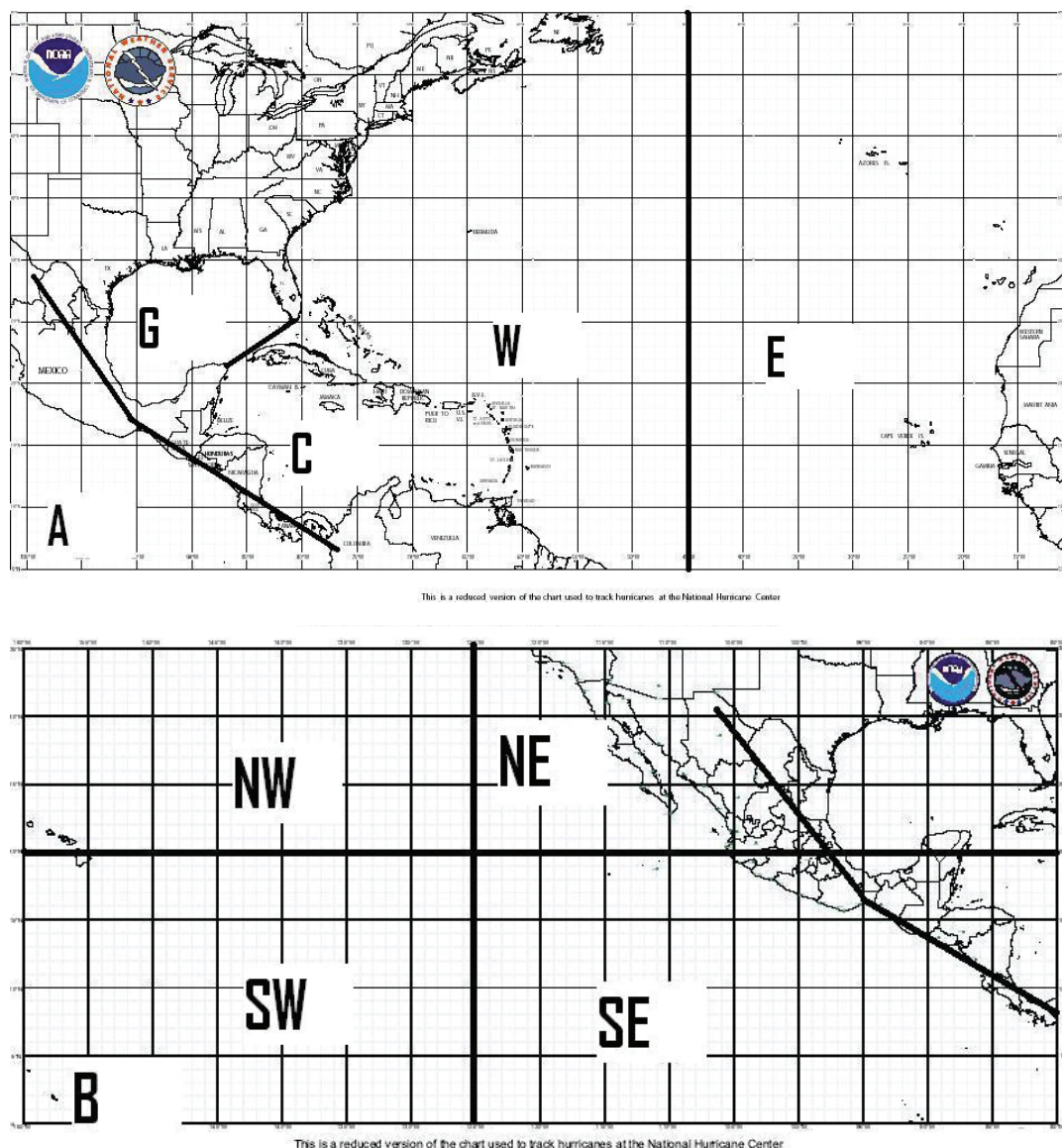
Fig. 1. The maps of a) the Atlantic Ocean Basin (G = Gulf, C = Caribbean, W (E) = West (East) Atlantic), and the b) Pacific Ocean Basin (NW = Northwest, NE = Northeast, SW= Southwest, and SE= Southeast) used in this study and provided by the National Hurricane Center. The heavy lines represent the boundaries between sub-basins used in this study. Their boundaries are outlined in section 2b and LJ00. The diagonal line across Mexico represents a dividing line between the Atlantic and Pacific Basins.
