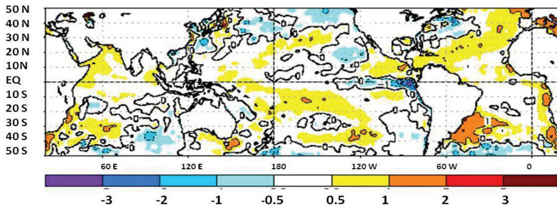
Fig. 8. As in Fig. 4, except for April 2007.
